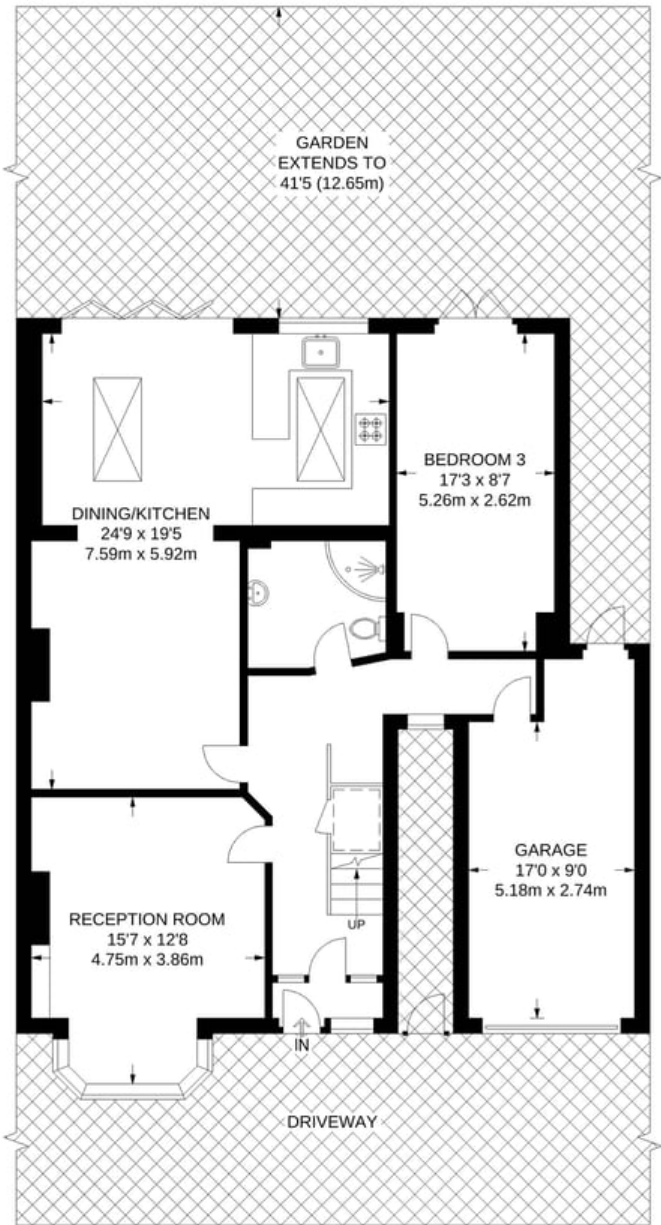
GROUND FLOOR 1088 SQ FT / 101.1 SQ M
